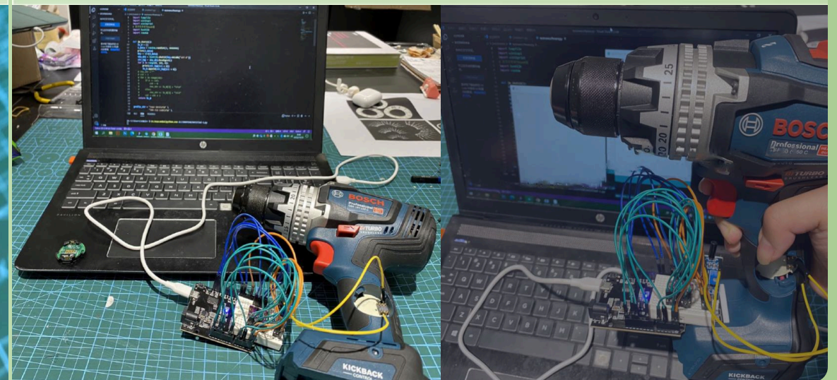
Bluetooth Module Enhancement Design (Arduino Demo)
